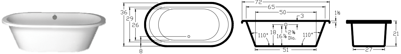
All bathtub dimensions are ± 1/2".
